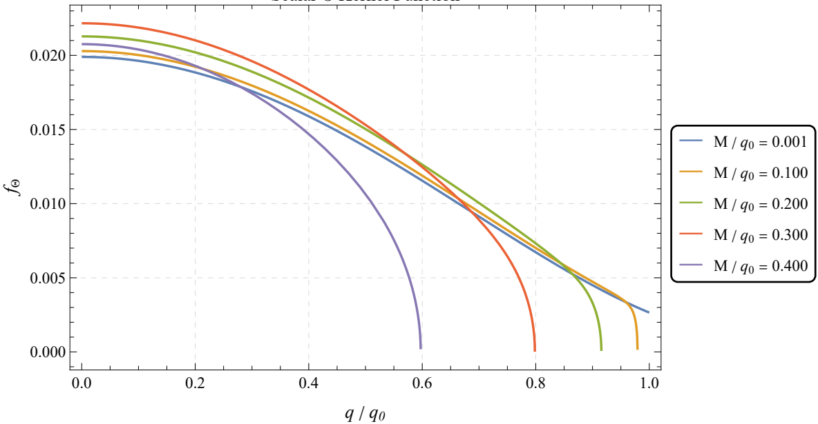
Scalar \Theta Kernel Function
